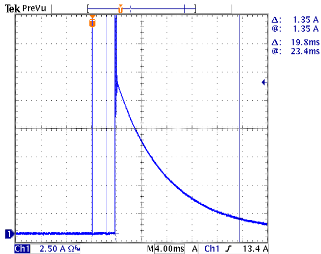
EBM-1K2S350DG ( I_o=2600mA )
