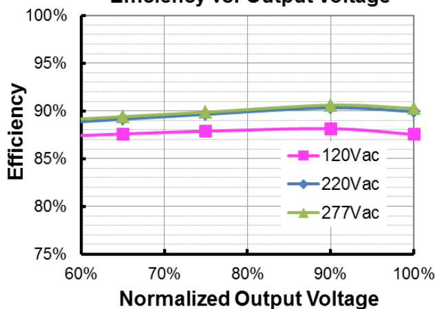
EUM-075S105Lx (Io=700mA) Efficiency vs. Output Voltage
