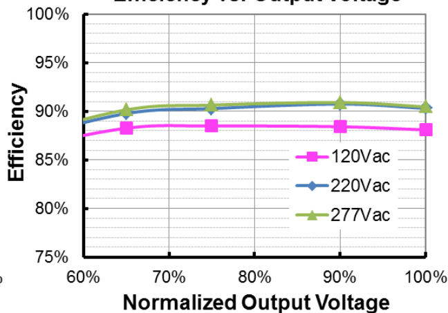
EUM-075S105Lx (Io=1050mA) Efficiency vs. Output Voltage
