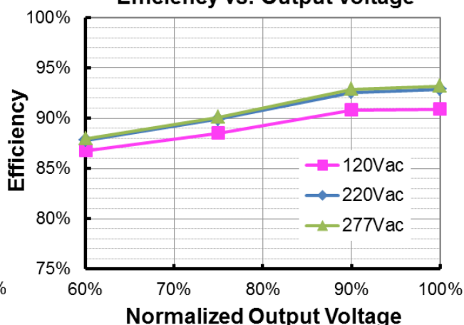
EUM-150S210Mx(I o =2100mA) Efficiency vs. Output Voltage
