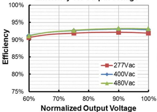
ESM-240S350Lx ( I_o=2150mA ) Efficiency vs. Output Voltage
