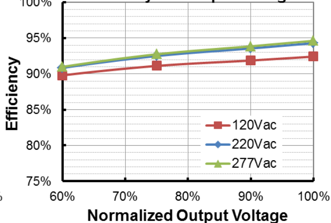
EUM-320S150Lx (I o =1500mA) Efficiency vs. Output Voltage
