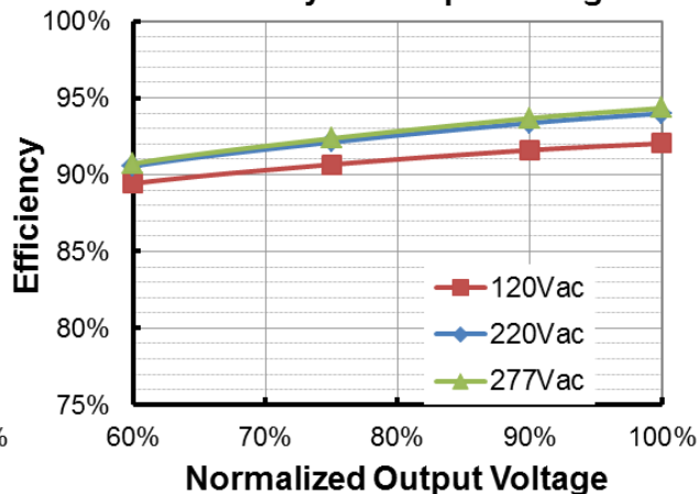
EUM-320S250Lx (I o =2500mA) Efficiency vs. Output Voltage
