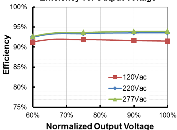
EUM-320S500Lx (I o =2850mA) Efficiency vs. Output Voltage
