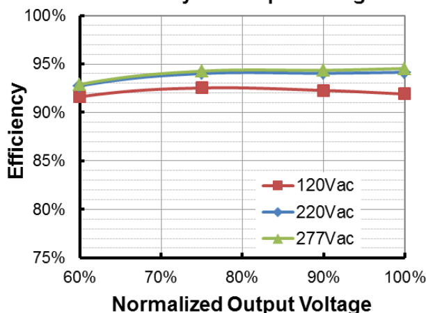
EUM-320S250Lx (I o =1750mA) Efficiency vs. Output Voltage
