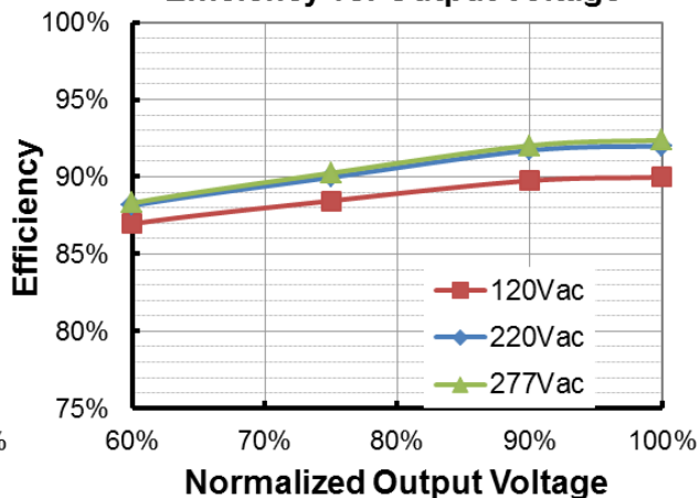
EUM-320S500Lx (I o =5000mA) Efficiency vs. Output Voltage
