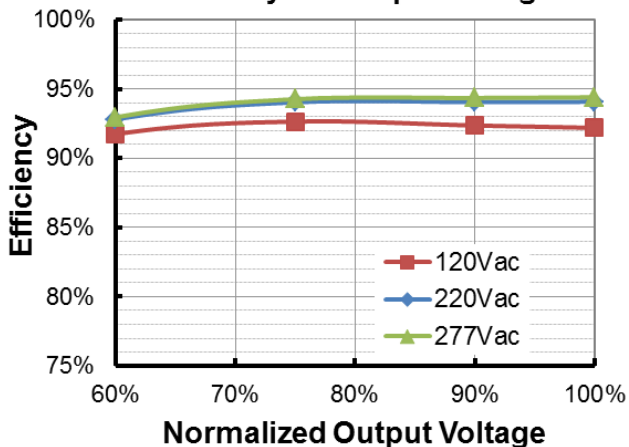
EUM-320S150Lx (I o =1050mA) Efficiency vs. Output Voltage
