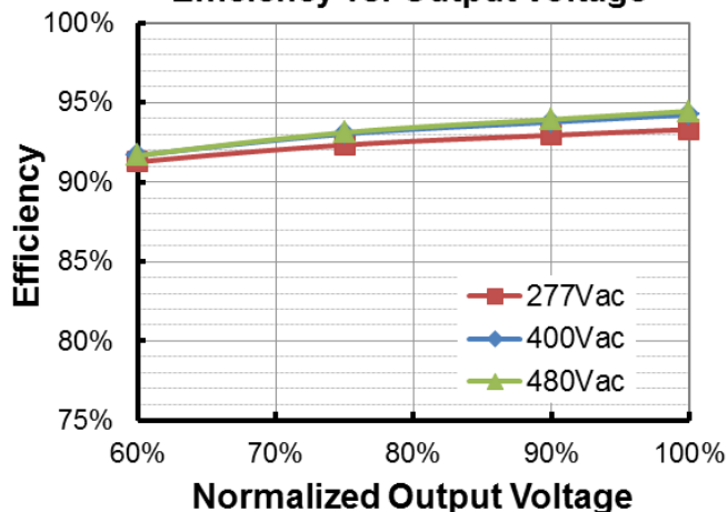
ESM-680S240Mx( I_o=2400\text{mA} ) Efficiency vs. Output Voltage
