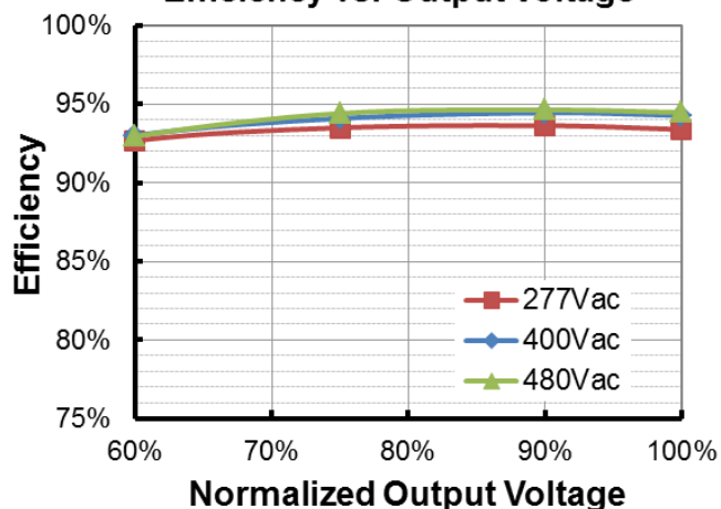
ESM-680S15AMx( I_o=12600\text{mA} ) Efficiency vs. Output Voltage
