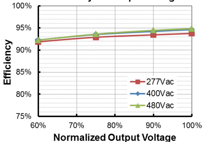
ESM-680S170Mx( I_o=1700\text{mA} ) Efficiency vs. Output Voltage
