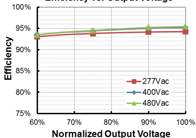
ESM-680S240Mx( I_o=1800\text{mA} ) Efficiency vs. Output Voltage
