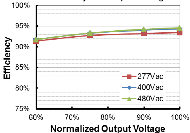
ESM-680S15AMx( I_o=15000\text{mA} ) Efficiency vs. Output Voltage
