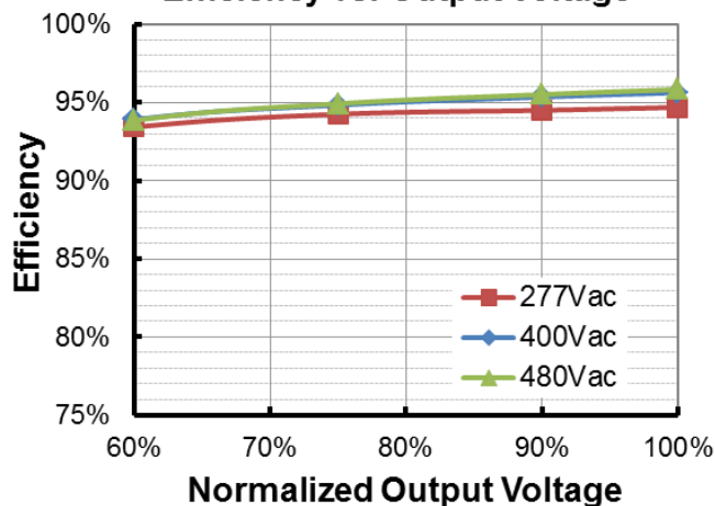
ESM-680S170Mx( I_o=1250\text{mA} ) Efficiency vs. Output Voltage
