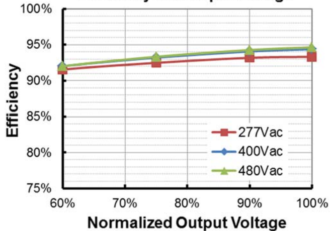
ESM-680S560Mx(I o =5600mA) Efficiency vs. Output Voltage
