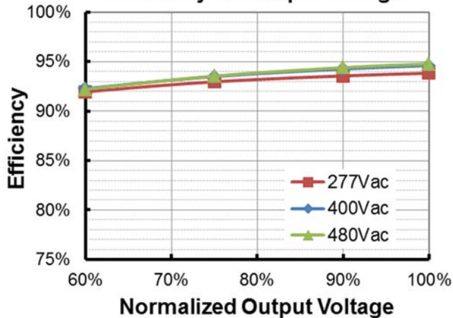
ESM-680S350Mx(I o =3500mA) Efficiency vs. Output Voltage
