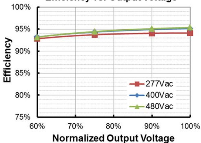
ESM-680S15AMx( I_o=12600\text{mA} ) Efficiency vs. Output Voltage
