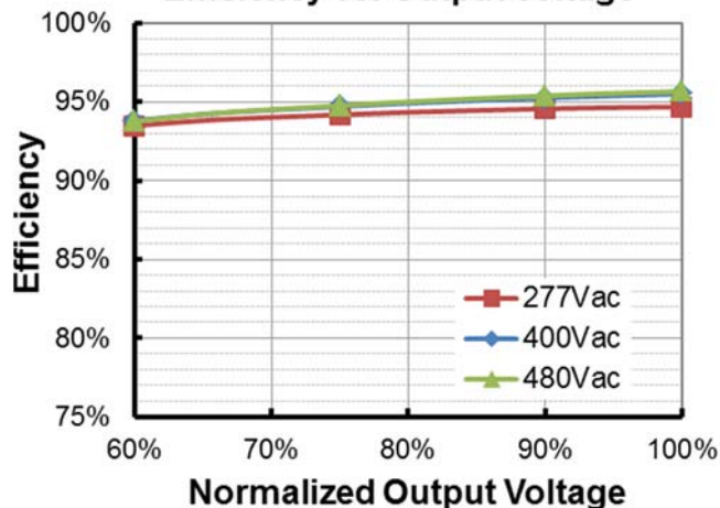
ESM-680S350Mx(I o =2600mA) Efficiency vs. Output Voltage
