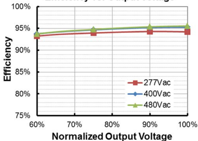
ESM-680S560Mx(I o =4200mA) Efficiency vs. Output Voltage
