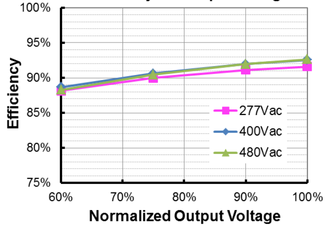
ESM-150S150Bx( I_o=1500mA ) Efficiency vs. Output Voltage
