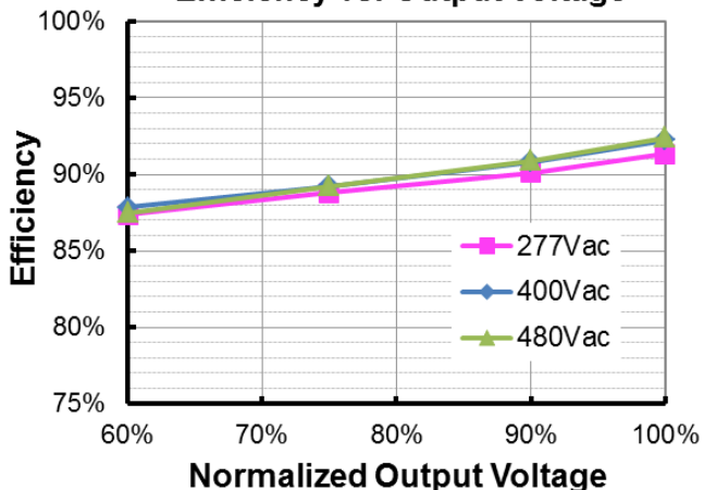
ESM-150S420Bx( I_o=4200mA ) Efficiency vs. Output Voltage
