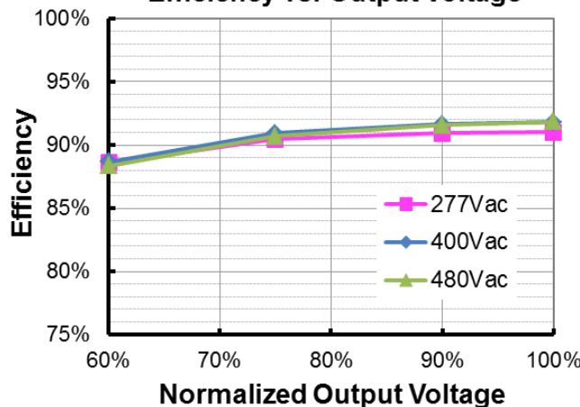
ESM-150S420Bx( I_o=2800mA ) Efficiency vs. Output Voltage
