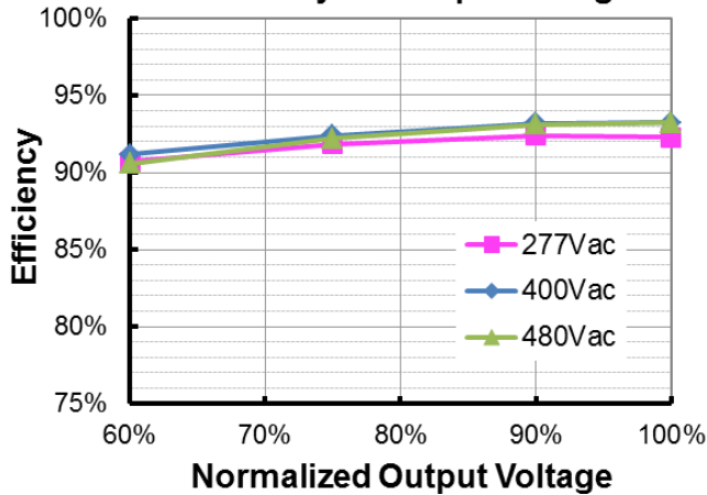
ESM-150S150Bx( I_o=1050mA ) Efficiency vs. Output Voltage
