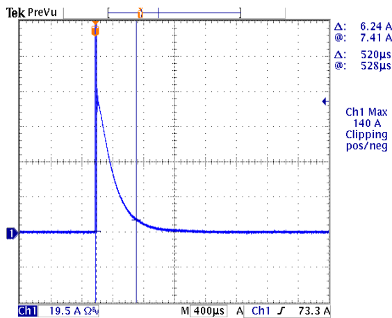
ESM-240S105Mx( I_o=1050mA )
