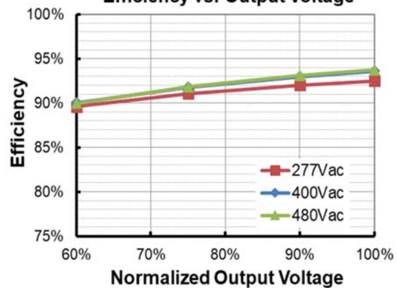
ESM-240S150Mx( I_o=1500mA )
