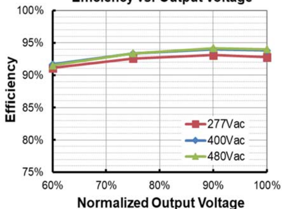
ESM-240S670Mx( I_o=4200\text{mA} ) Efficiency vs. Output Voltage
