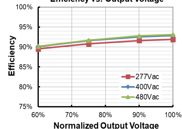
ESM-320S760Mx( I_o=7600mA ) Efficiency vs. Output Voltage
