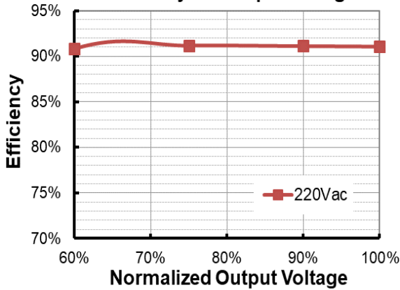
EBS-080S150DT2 (Io=1050mA) Efficiency vs. Output Voltage
