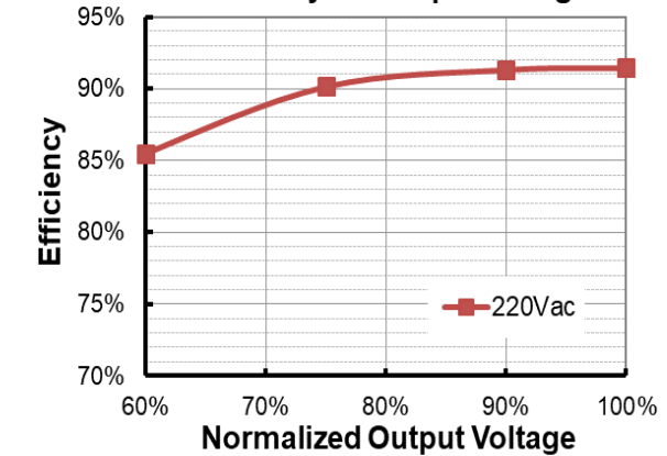
EBS-080S150DT2 (Io=1500mA) Efficiency vs. Output Voltage
