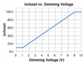
Implementation 3: Positive logic
