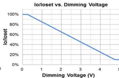
Implementation 2: Negative logic
