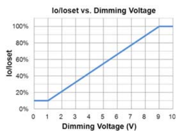
Implementation 3: Positive logic
