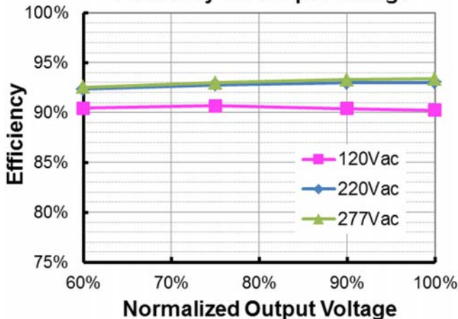
EUM-240S350Bx ( I_o=2150mA ) Efficiency vs. Output Voltage
