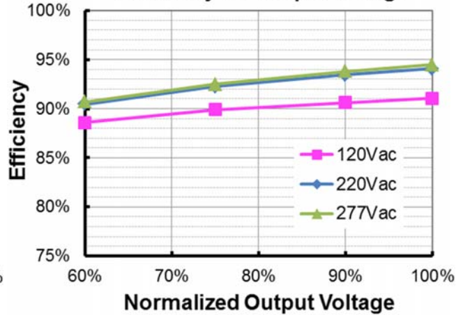
EUM-240S150Bx ( I_o=1500mA ) Efficiency vs. Output Voltage
