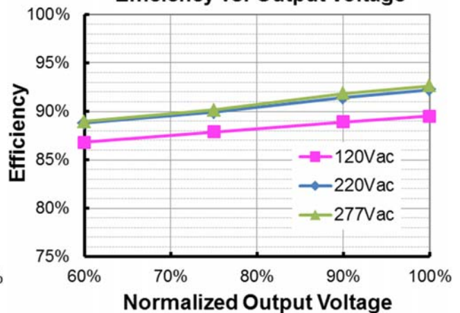
EUM-240S350Bx ( I_o=3500mA ) Efficiency vs. Output Voltage
