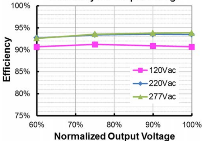
EUM-240S150Bx ( I_o=1050mA ) Efficiency vs. Output Voltage
