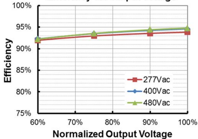
ESM-680S350BG(I o =3500mA) Efficiency vs. Output Voltage
