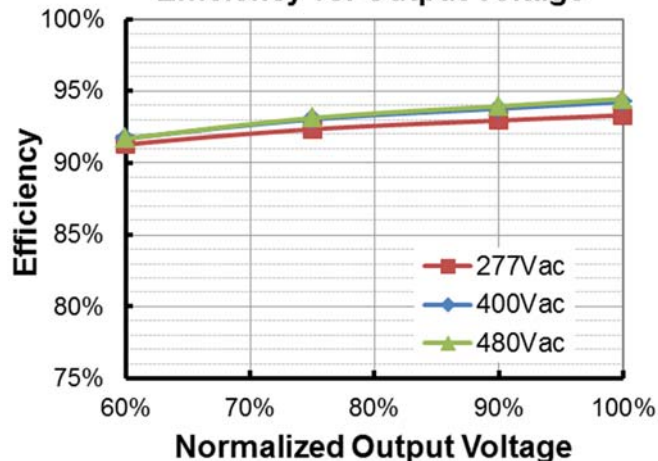
ESM-680S240BG(I o =2400mA) Efficiency vs. Output Voltage
