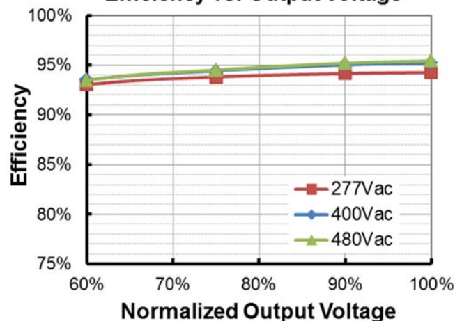
ESM-680S240BG(I o =1800mA) Efficiency vs. Output Voltage
