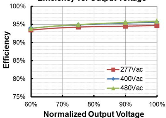
ESM-680S240BG(I o =1800mA) Efficiency vs. Output Voltage
