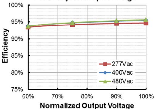
ESM-680S350BG(I o =2600mA) Efficiency vs. Output Voltage
