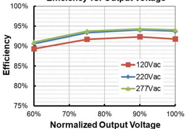
SUM-220S530HF (Io=4100mA) Efficiency vs. Output Voltage
