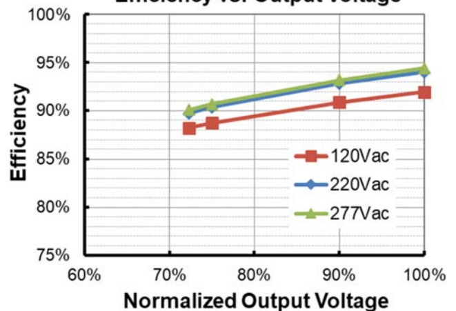
SUM-220S530HF (Io=5300mA) Efficiency vs. Output Voltage
