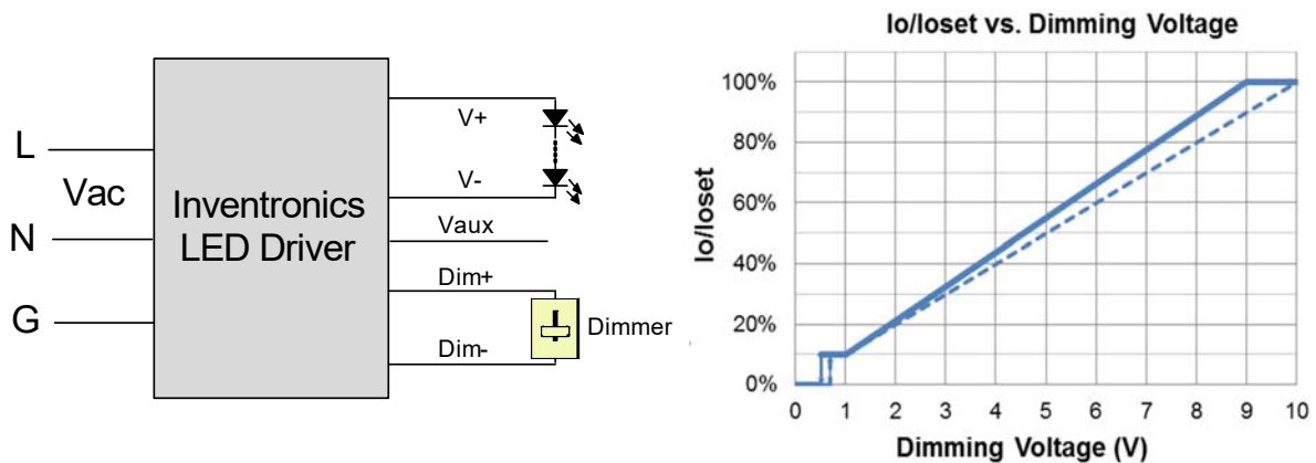
Implementation 1: Positive logic
