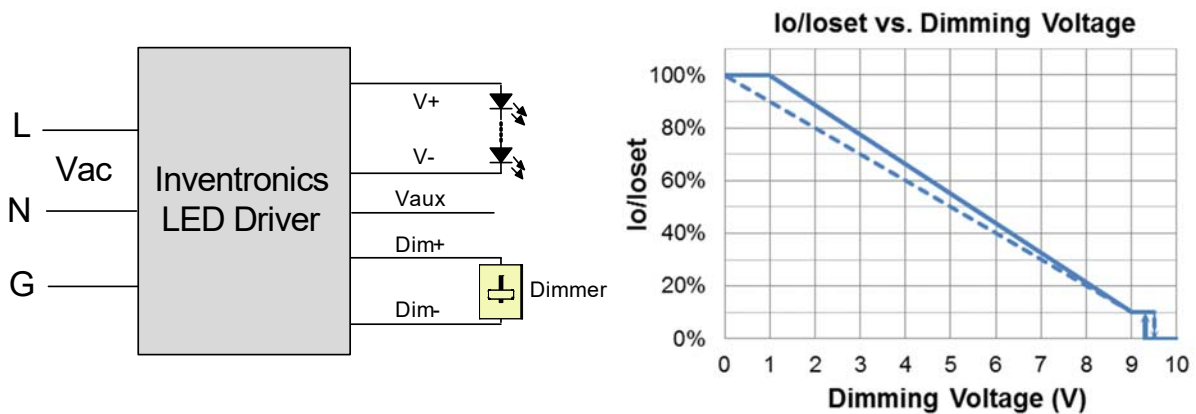
Implementation 2: Negative logic
