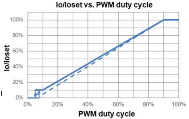
Implementation 3: Positive logic
