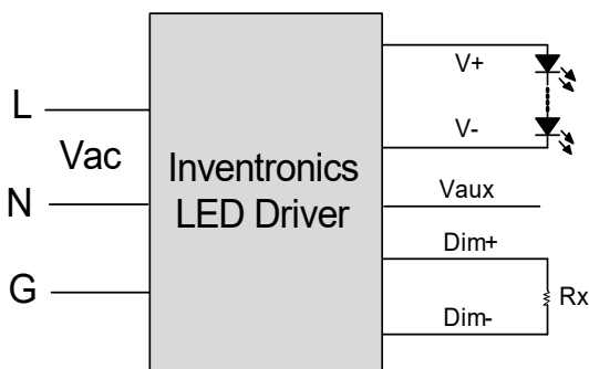
Implementation 5: Positive logic
