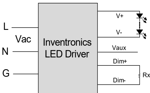
Implementation 6: Negative logic
