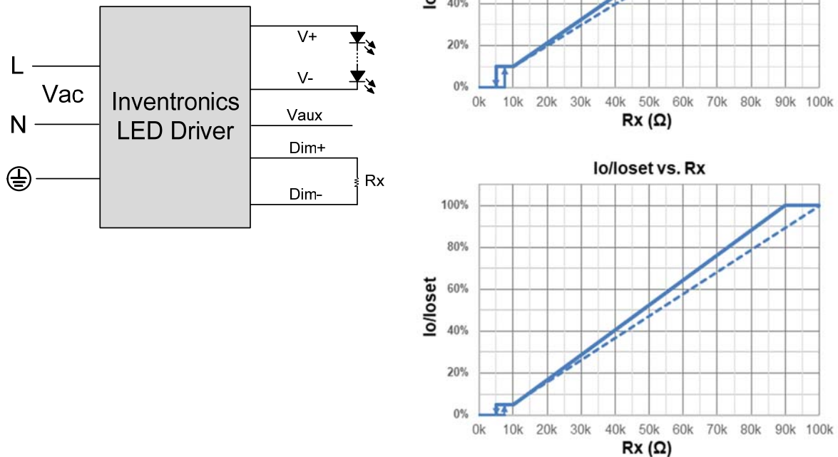
Implementation 5: Positive logic
