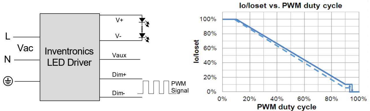
Implementation 4: Negative logic
