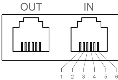
RJ12 Connector
