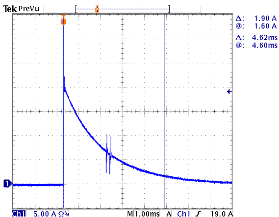
ESM-320S105Mx( I_o=1050mA )
