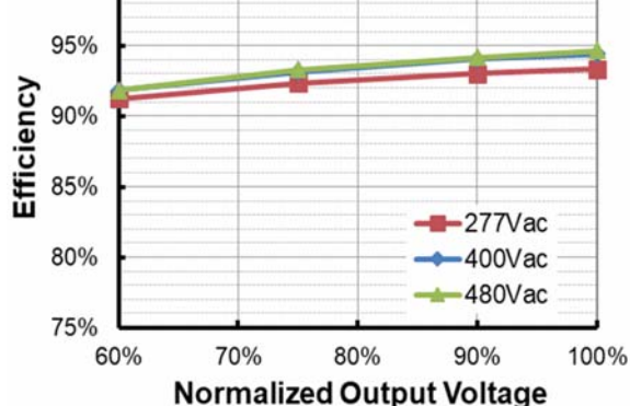
Efficiency vs. Output Voltage
