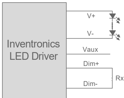
Implementation 6: Negative logic
