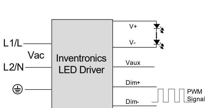
Implementation 4: Negative logic
