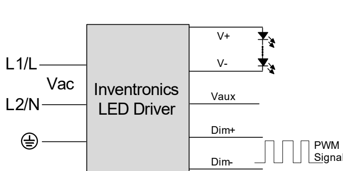
Implementation 3: Positive logic
