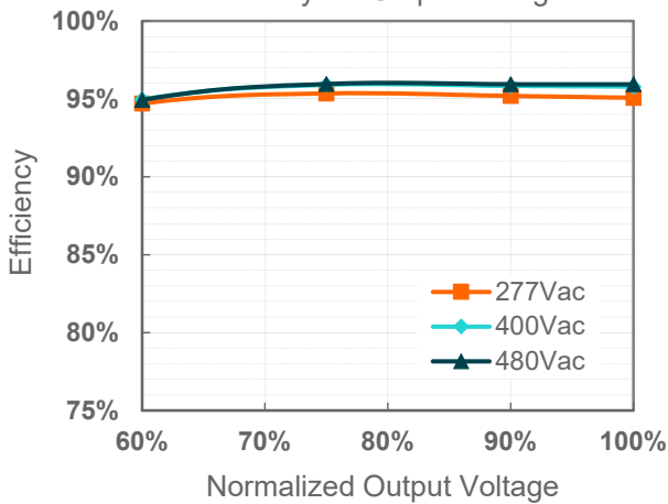
ESM-880S420Mx( I_o=3000mA ) Efficiency vs. Output Voltage
