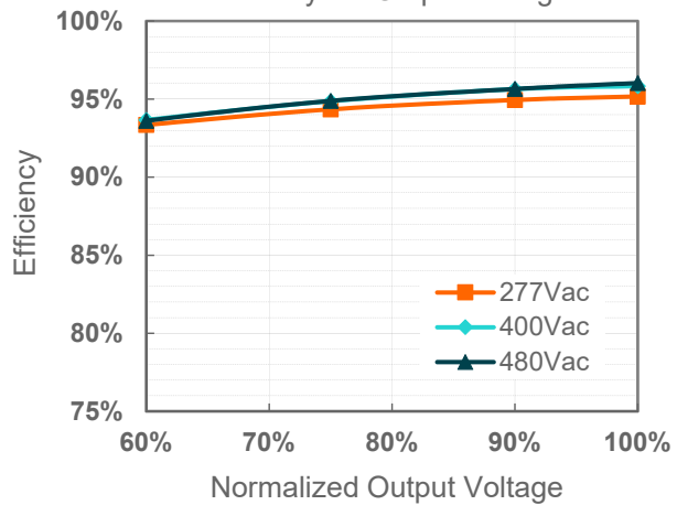
ESM-880S420Mx( I_o=4200mA ) Efficiency vs. Output Voltage
