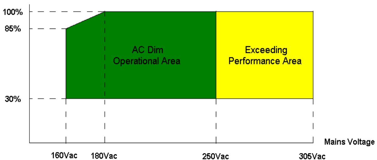
Output Level
