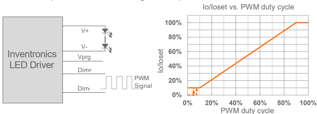
Implementation 4: Positive logic
