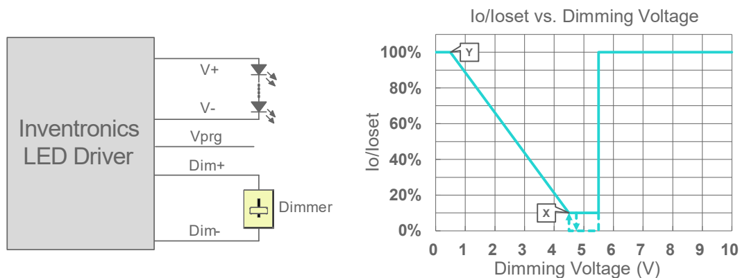
Implementation 6: Negative logic
