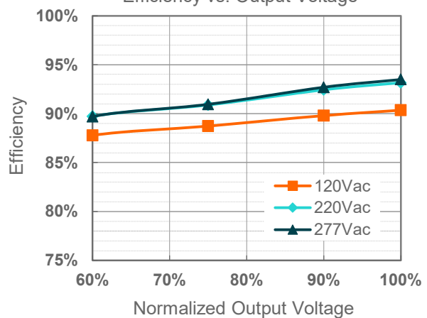
EUM-240S150Mx(I o =1500mA) Efficiency vs. Output Voltage
