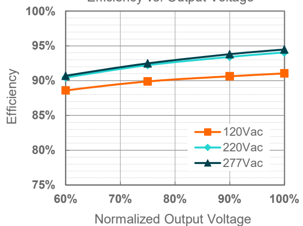
EUM-240S105Mx(I o =1050mA) Efficiency vs. Output Voltage
