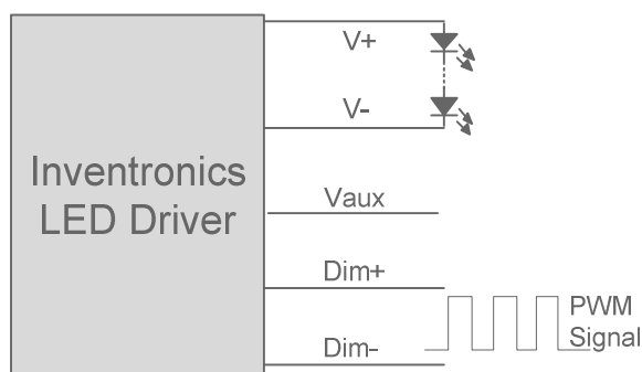
Implementation 4: Negative logic
