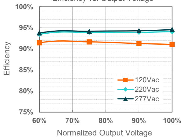
EUM-240S105Mx(I o =700mA) Efficiency vs. Output Voltage
