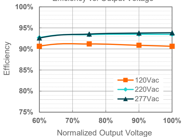
EUM-240S150Mx(I o =1050mA) Efficiency vs. Output Voltage
