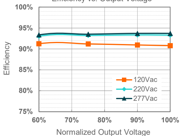
EUM-200S150Bx(I o =1050mA)
