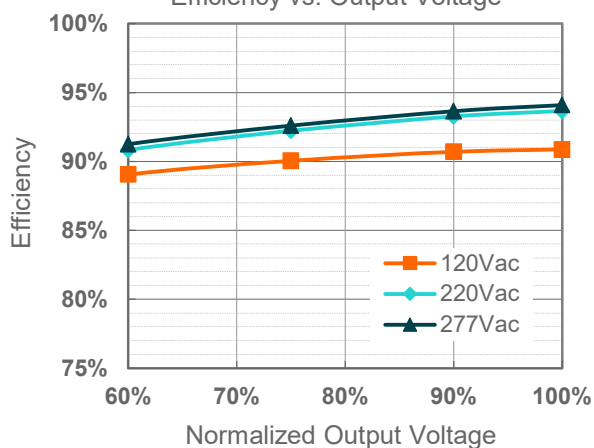
EUM-200S150Bx(I o =1500mA)
